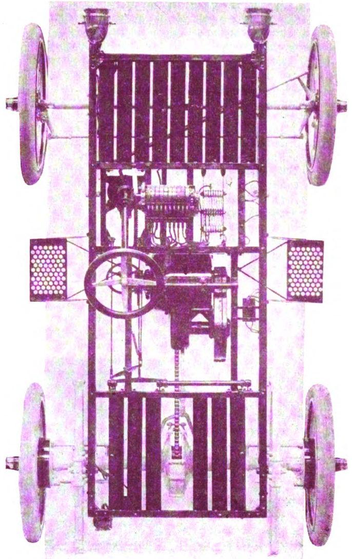
Baker Chassis Complete Allows of Body Choices.
